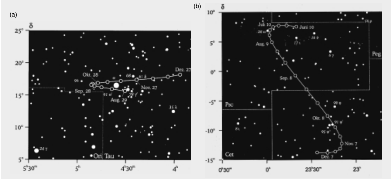
FIGURE 2.9. Star charts show apparent retrograde motion for the asteroids (a) Ceres, and (b) Pallas, during 1998.
